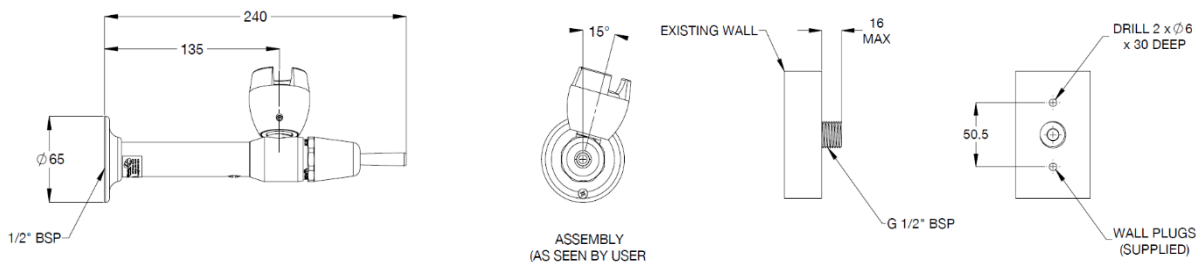
Rough-in Dimensions
